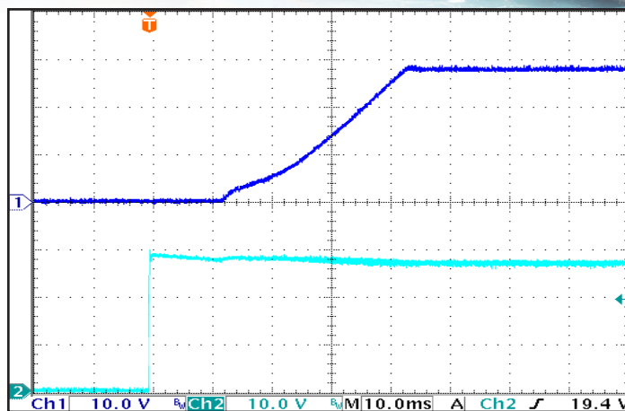
Figure 8: Turn-On Transient , at full resistive load and zero output capacitance, initiated by Vin. Ch 1: Vout (10 V/div); Ch 2: Vin (10 V/div).
