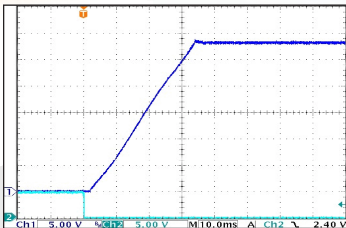
Figure 7: Typical Startup Waveform , input voltage pre-applied. Ch 1: Vout (5 V/div); Ch 2: ON/OFF Pin (5 V/div).
