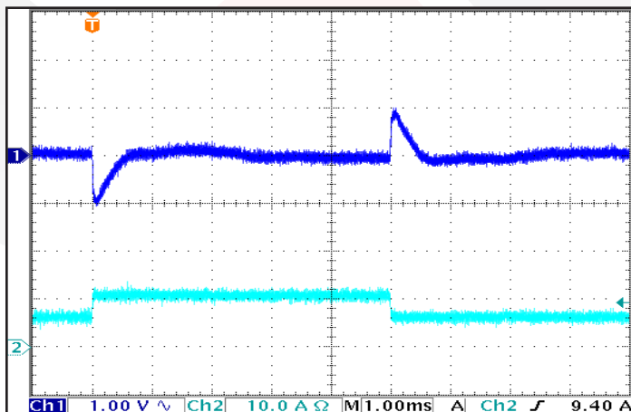
Figure 11: Output Voltage Response to Step-Change in Load Current , (50%-75%-50% of Iout(max); di/dt = 5 A/ \mu s). Load capacitance: 1 \mu F ceramic and 100 \mu F electrolytic capacitors. Ch 1: \Delta Vout (1 V/div); Ch 2: Iout (10 A/div).
