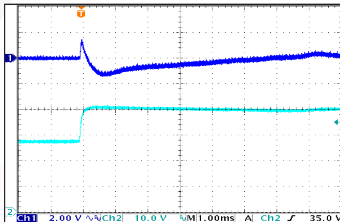
Figure 12: Output Voltage Response to Step-Change in Input Voltage , ( dV/dt = 250 V/ms). Load capacitance: 1 \mu F ceramic and 1000 \mu F electrolytic capacitors. Ch 1: Vout (2 V/div); Ch 2: \Delta Vin (10 V/div).
