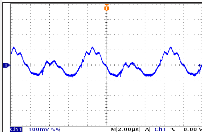
Figure 10: Output Voltage Ripple , Vout, at nominal input voltage and rated load current (100 mV/div). Load capacitance: 1 \mu F ceramic and 100 \mu F electrolytic capacitors. Bandwidth: 20 MHz. See Figure 13.
